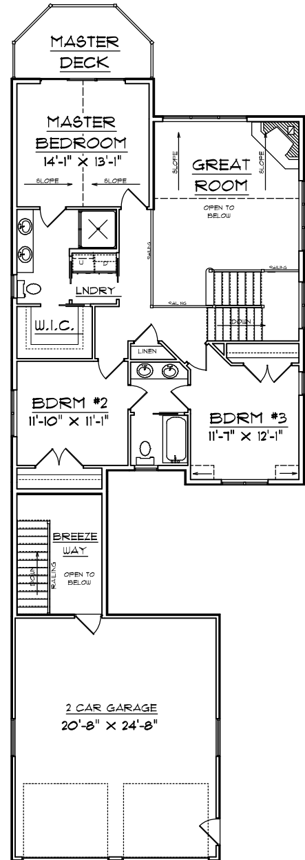
2ND FLOOR PLAN
