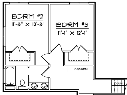
2ND FLOOR PLAN
