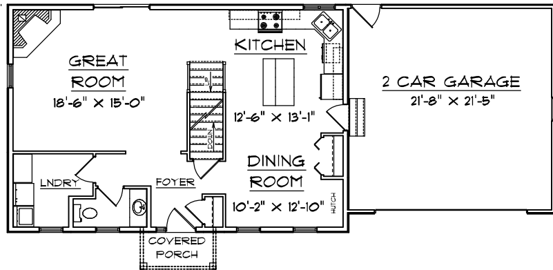
1ST FLOOR LAYOUT
