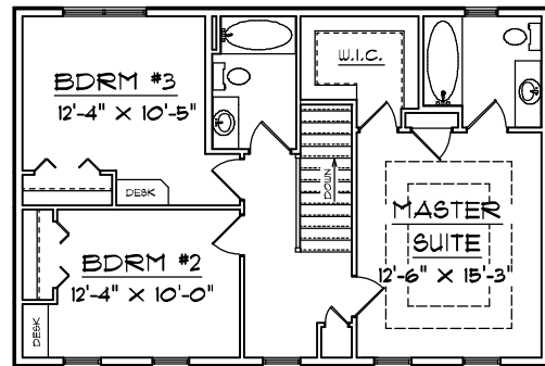
2ND FLOOR LAYOUT
