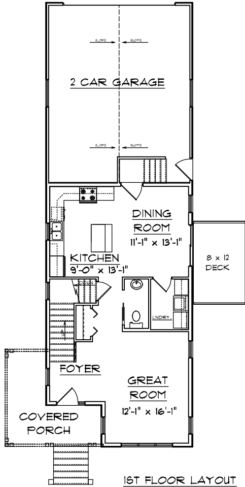
1ST FLOOR LAYOUT
