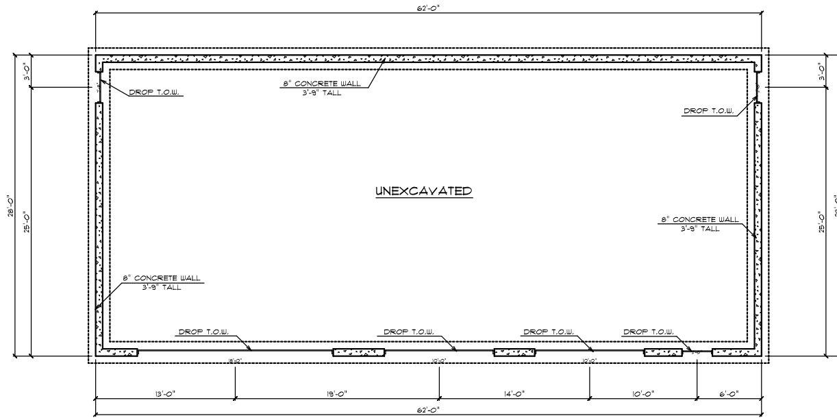
FOUNDATION PLAN SCALE: 1/4" = 1'-0"
