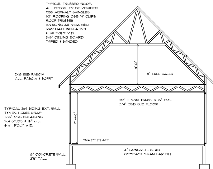
SECTION THROUGH NO SCALE
