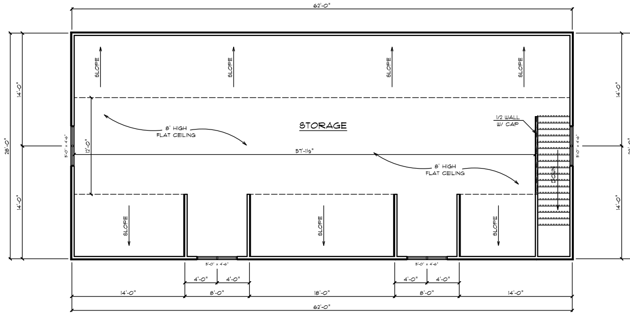
UPPER FLOOR LAYOUT SCALE: 1/4" = 1'-0"
