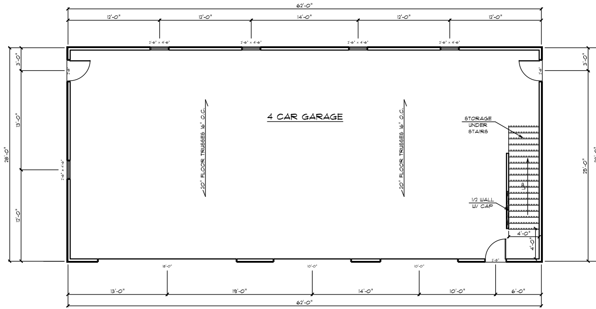
MAIN FLOOR LAYOUT SCALE: 1/4" = 1'-0"
