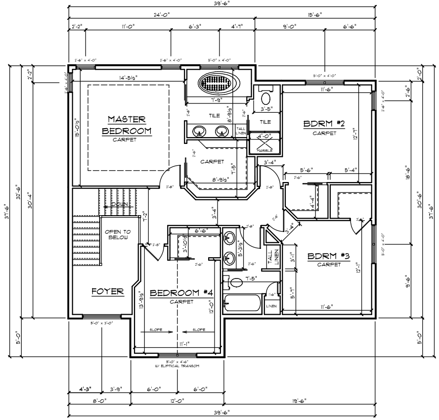
2ND FLOOR PLAN SCALE: 1/4" = 1'-0" 1135 SQFT
