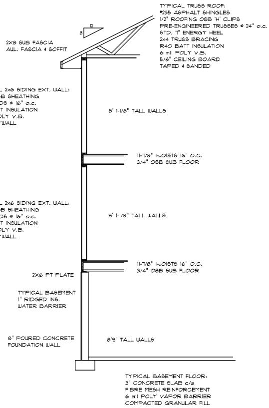
CROSS SECTION NO SCALE
