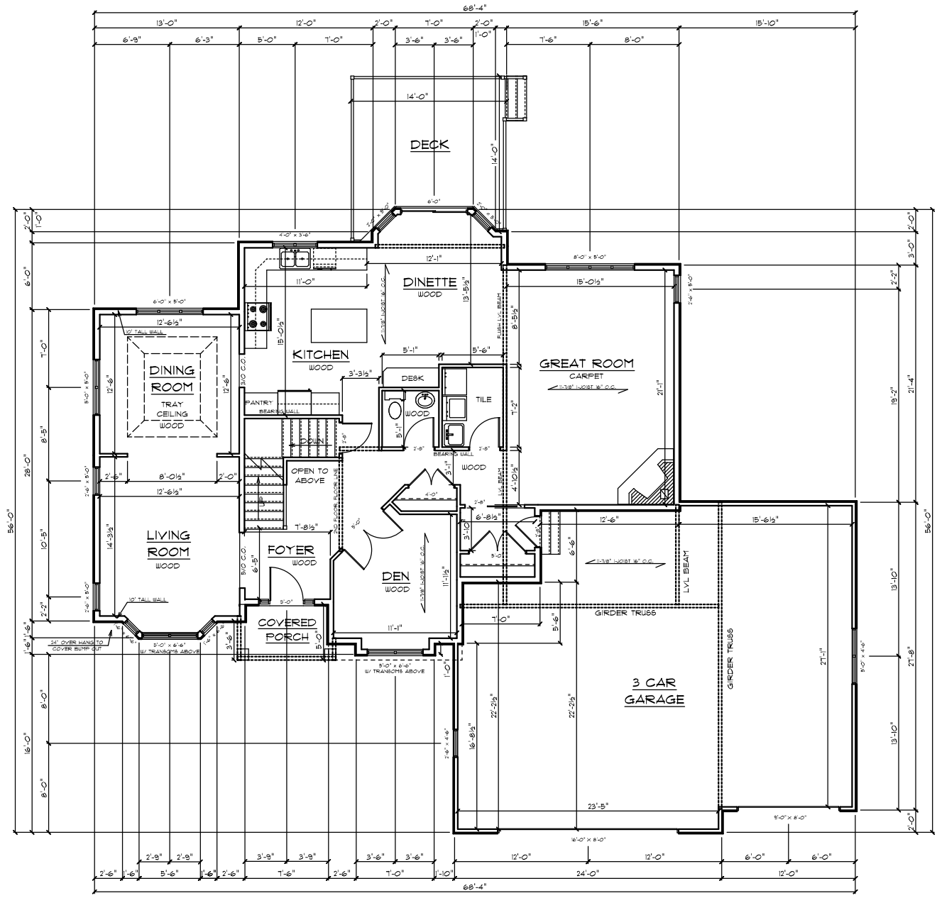
1ST FLOOR PLAN SCALE: 1/4" = 1'-0" 1587 SQFT
