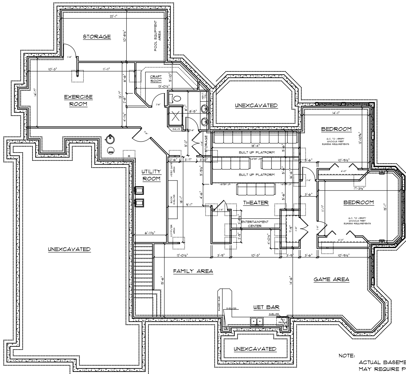
BASEMENT FINISH PLAN SCALE: 1/4" = 1'-0" 2560 SQFT FINISHED AREA
